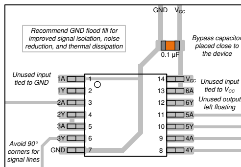
Figure 9. Example layout for the SN74HC04-Q1
