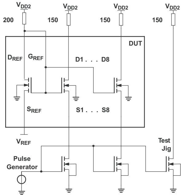
Figure 7-2. Load Circuit
