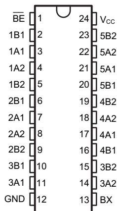
Pin Functions
