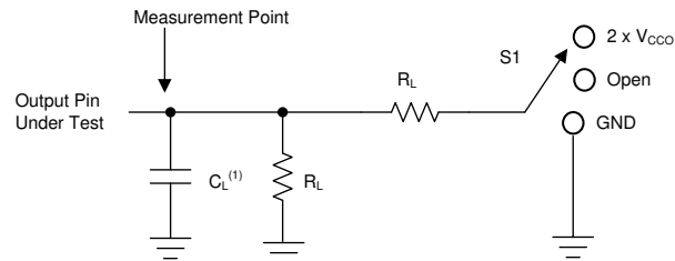
Figure 1. Load Circuit
