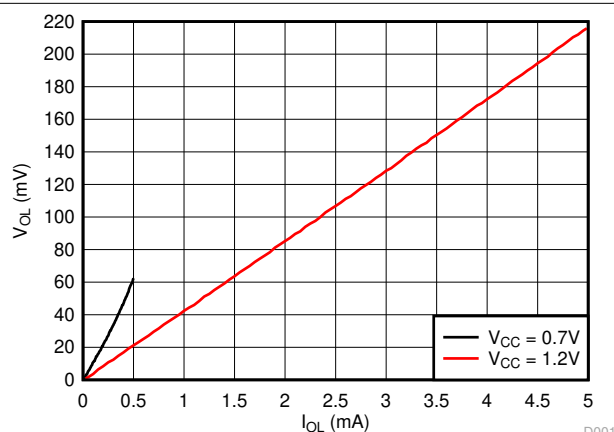
Figure 5-4. Typical ( T_A=25^\circ\text{C} ) Output High Voltage ( V_{OL} ) vs Sink Current ( I_{OL} )
