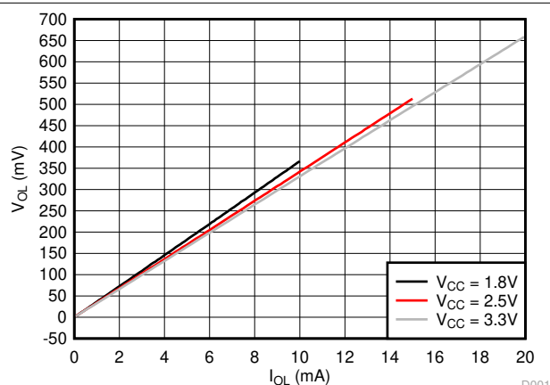
Figure 5-3. Typical ( T_A=25^\circ\text{C} ) Output High Voltage ( V_{OL} ) vs Sink Current ( I_{OL} )
