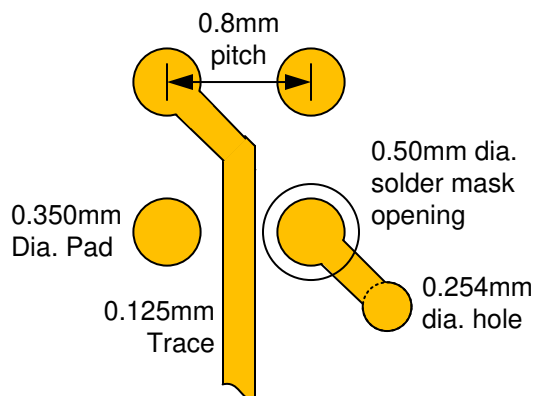
Figure 11-1. BGA Layout Example
