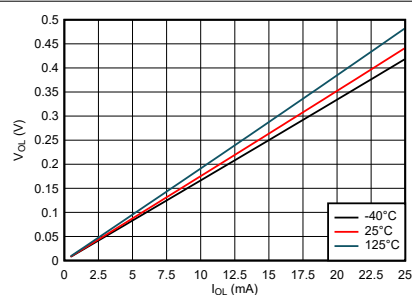
Figure 6-2. Output Voltage vs Current in LOW State
