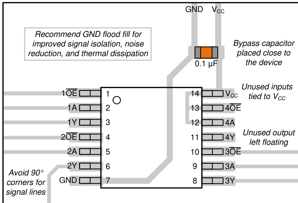
Figure 9-3. Example Layout for the SN74AHCT125-Q1
