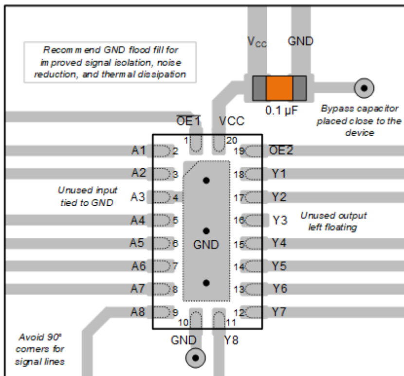
Figure 8-1. Layout Diagram
