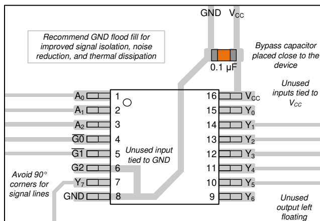
Figure 8-3. Example Layout for the SN74AHC238-Q1
