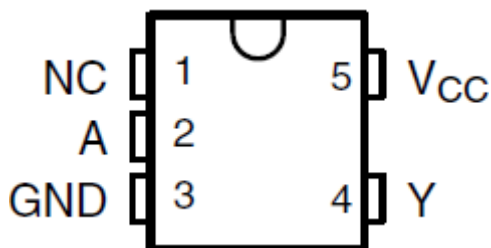
Figure 4-1. DBV or DCK Package (Top View)
