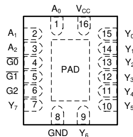
Figure 4-2. WBQB Package, 16-Pin WQFN (Top View)
