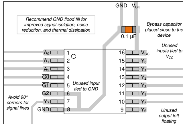
Figure 8-3. Example Layout for the SN74AHC138-Q1
