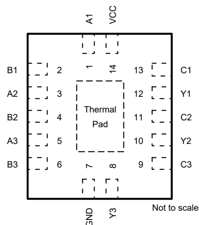
Figure 4-2. SN74ACT3G97 BQA Package, 14-Pin WQFN (Top View)
