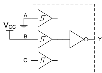
Schmitt-trigger inverter
