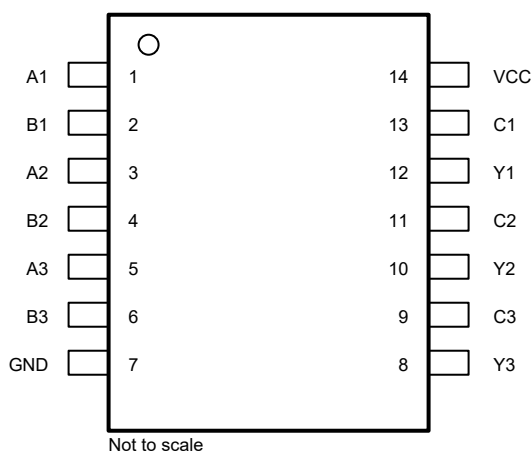
Figure 4-1. SN74ACT3G97 PW Package, 14-Pin TSSOP (Top View)
