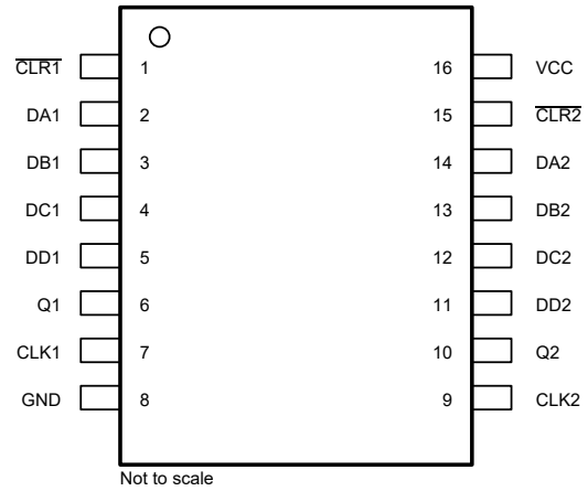
Figure 4-2. PW Package, 16-Pin TSSOP (Preview) (Top View)
