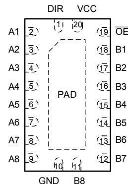
Figure 4-2. RKS Package, 20-Pin VQFN (Top View)
