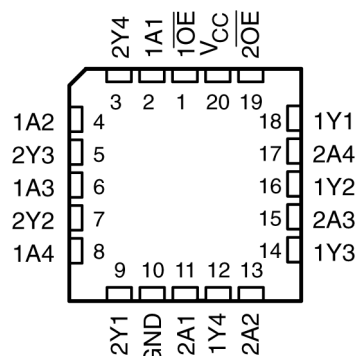
Figure 4-2. SN54ACT240 FK Package (Top View)
