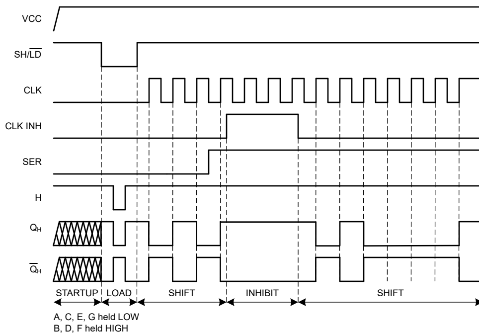
Figure 5-1. Timing Diagram
