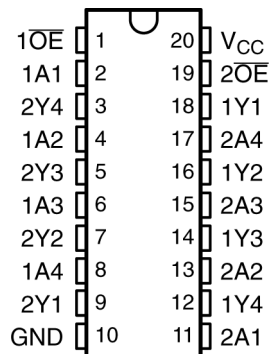
Figure 3-1. SN54AC241 DB, DW, N, NS, Or PW Package (Top View)
