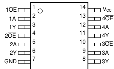
Figure 4-2. SN74AC126-Q1, PW Package (Top View)
