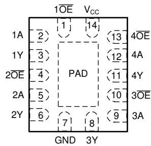
Figure 4-1. SN74AC126-Q1 BQA Package (Top View)
