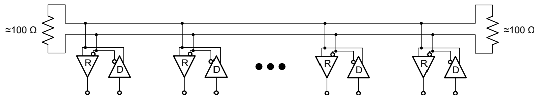
Figure 16. Multipoint Configuration
