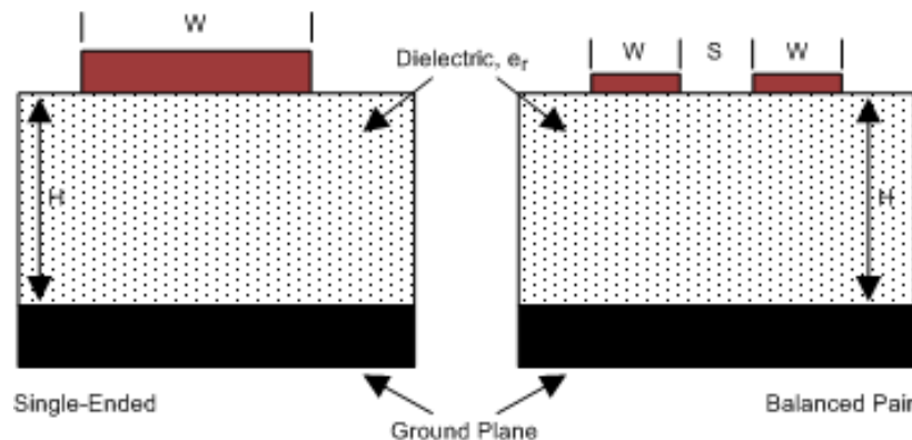
Figure 22. Microstrip Topology
