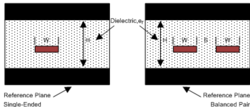
Figure 23. Stripline Topology
