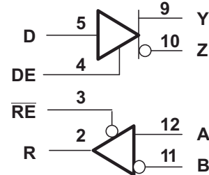
SN65MLVD202A, SN65MLVD205A
