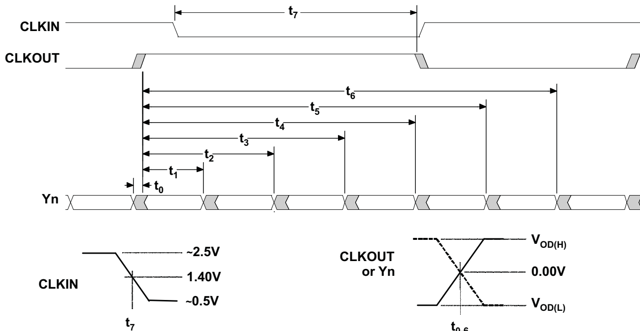
Figure 8. SN65LVDS93B-Q1 Timing Definitions
