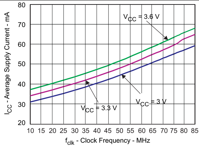
Figure 3. Average Grayscale I CC vs Clock Frequency
