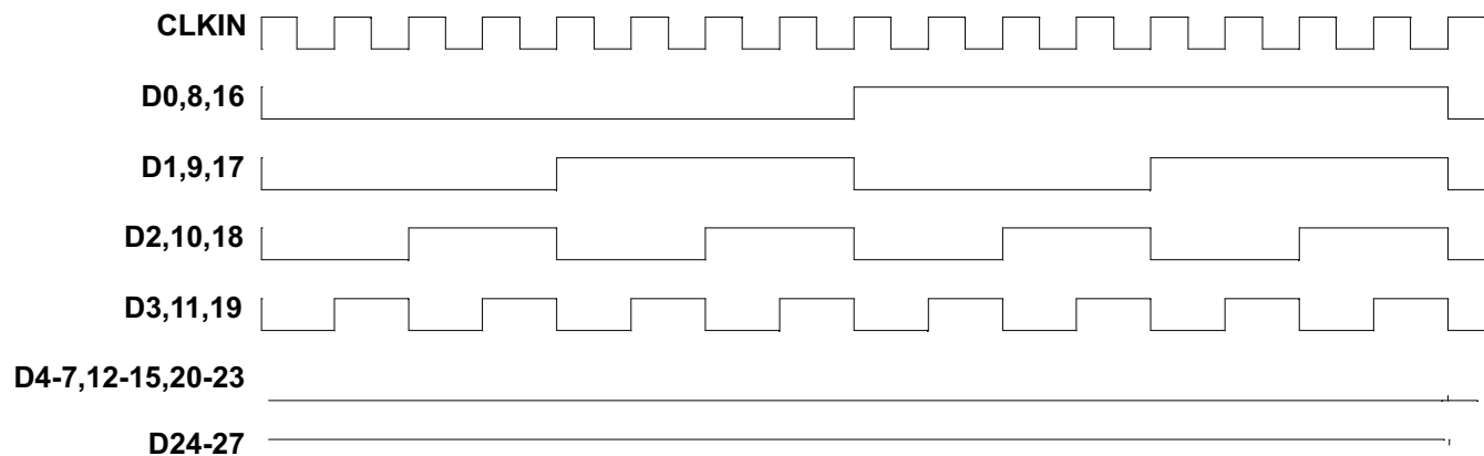
Figure 6. 16 Grayscale Test Pattern
