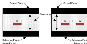
Figure 28. Stripline Topology
