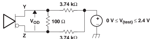
Figure 31. SN65LVDTx100 Differential Output Voltage ( V_{OD} ) Test Circuit
