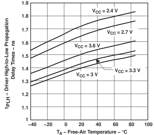
Figure 6-2. Driver Low-to-High Level Propagation Delay Times vs Free-Air Temperature
