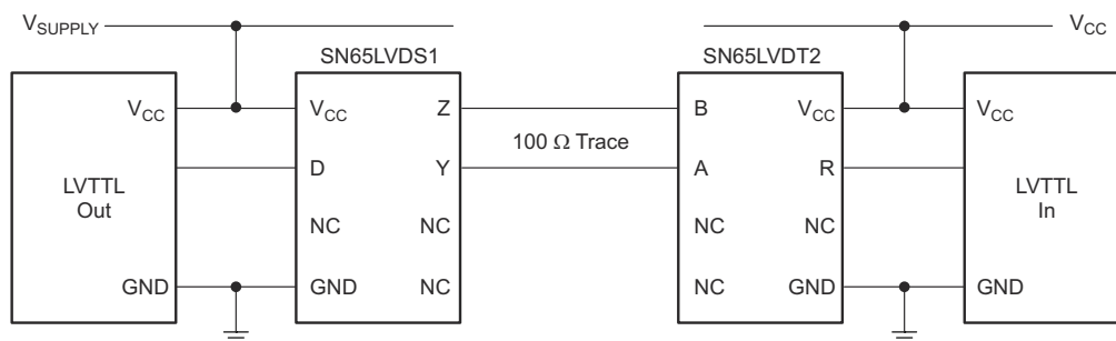
Simplified Schematic
