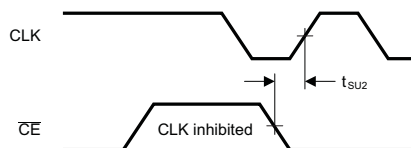
Figure 8. Serial – Shift Clock Inhibit Mode
