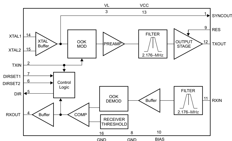
Block Diagram
