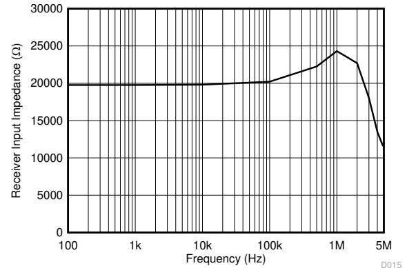
Figure 6-14. Receiver Input Impedance vs Frequency
