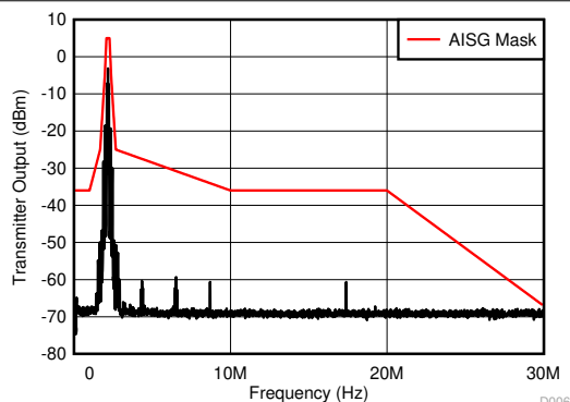
Figure 6-3. Low-Frequency Emissions Spectrum With 38.4-kbps Signaling Rate
