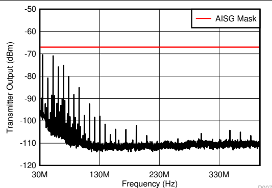
Figure 6-4. High-Frequency Emissions Spectrum With 38.4-kbps Signaling Rate
