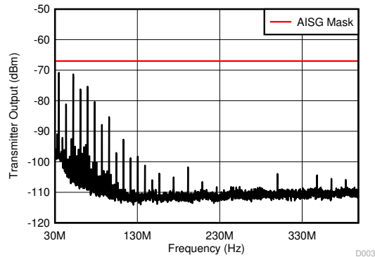
Figure 6-2. High-Frequency Emissions Spectrum With 9.6-kbps Signaling Rate
