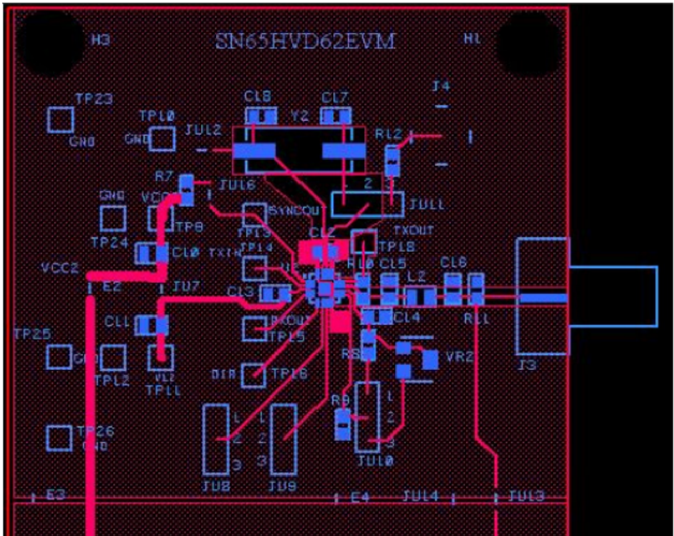
Figure 11-1. SN65HVD64 Layout
