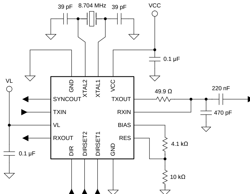
Figure 25. SN65HVD63 Schematic
