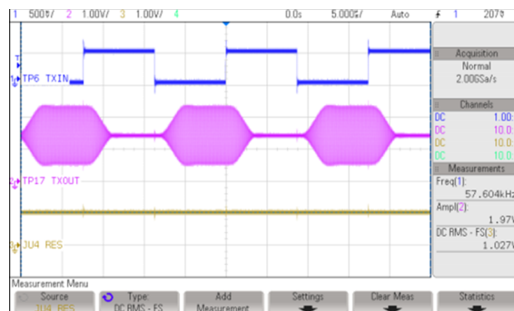
Figure 26. SN65HVD63 Application Curve
