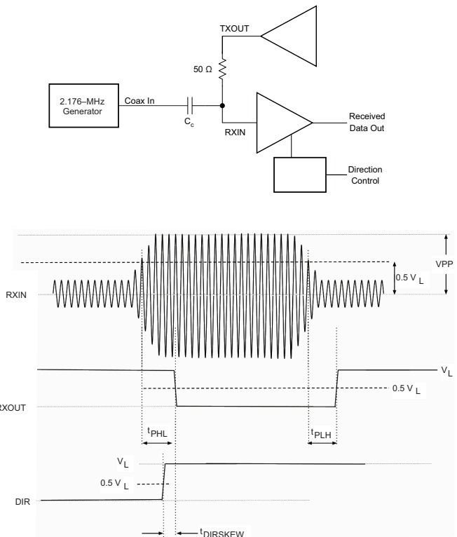
Figure 20. Measurement of Modem Receiver Propagation Delays
