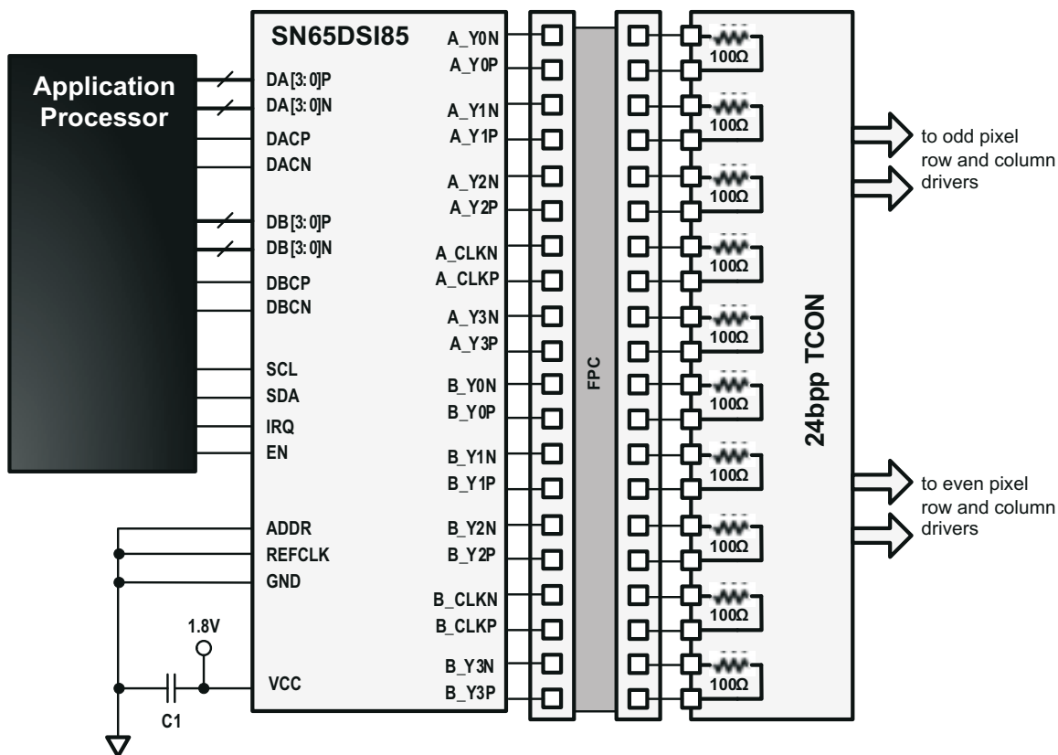
Figure 8-3. Typical WQXGA 24-bpp Panel Application
