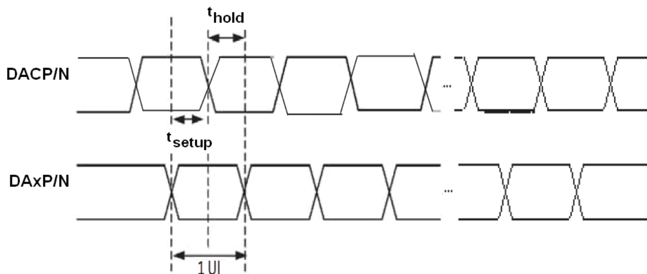
Figure 6-4. DSI HS Mode Receiver Timing Definitions
