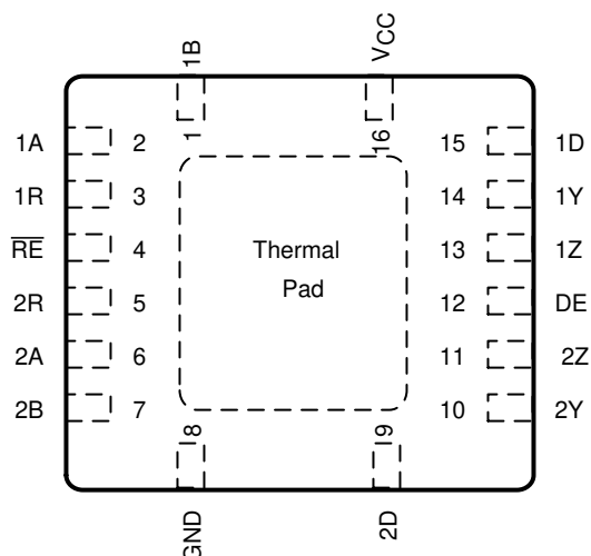
Figure 4-2. RGY Package 16 Pin (VQFN) Top View
