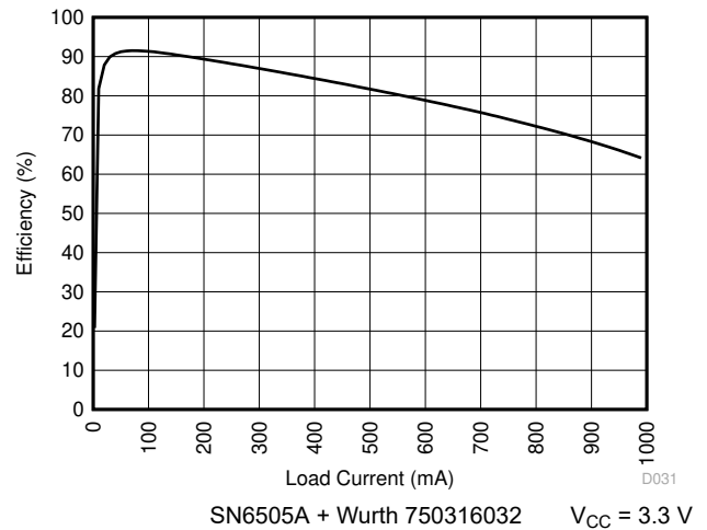
Figure 6-6. Efficiency vs Load Current
