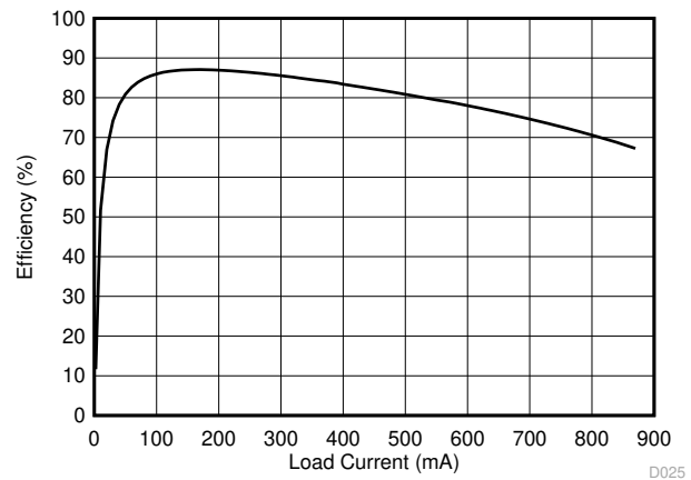
Figure 6-26. Efficiency vs Load Current
