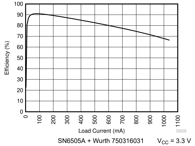
Figure 6-4. Efficiency vs Load Current
