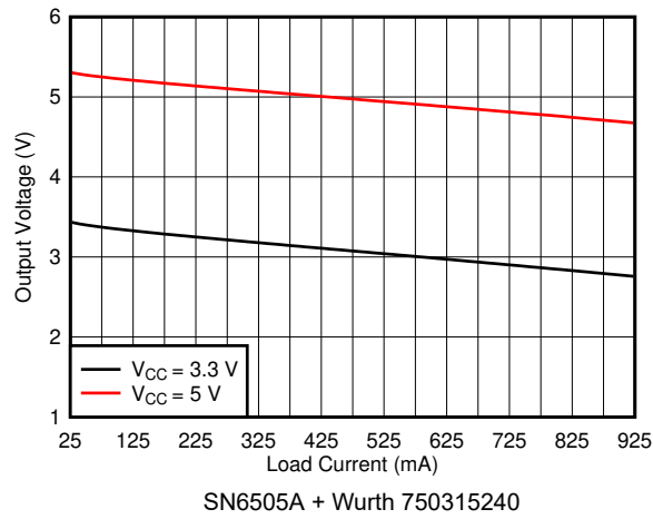
Figure 6-1. Output Voltage vs Load Current
