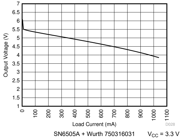
Figure 6-3. Output Voltage vs Load Current
