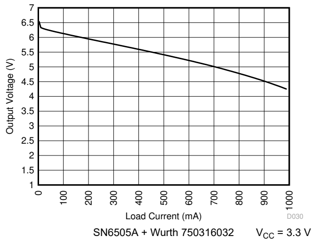
Figure 6-5. Output Voltage vs Load Current
