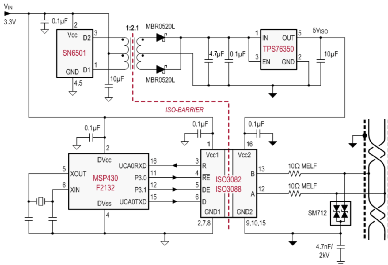
Figure 9-12. Isolated RS-485 Interface
