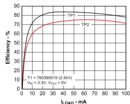
Figure 6-12. Efficiency vs Load Current
