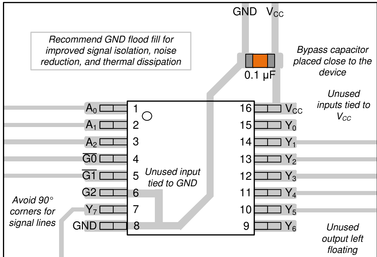
Figure 8-3. Example Layout for the SN54SC8T138-SEP
