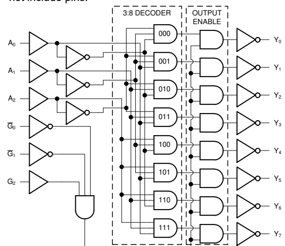
Simplified Logic Diagram (Positive Logic)
