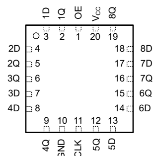
Figure 4-2. SN54AHCT374 FK Package (Top View)
