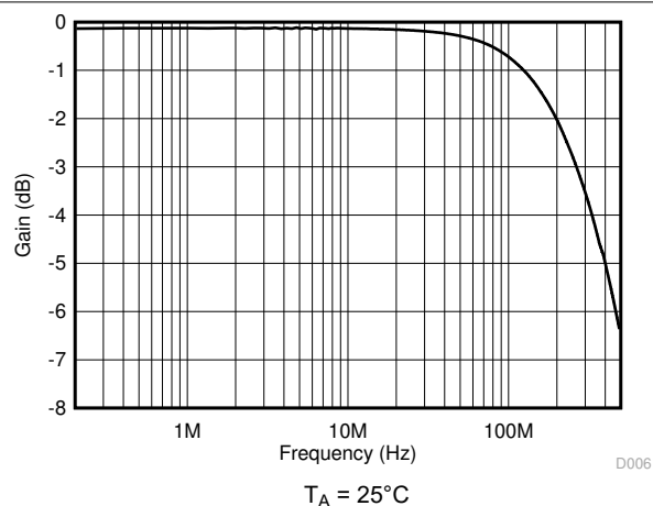
Figure 5-4. Frequency Response
