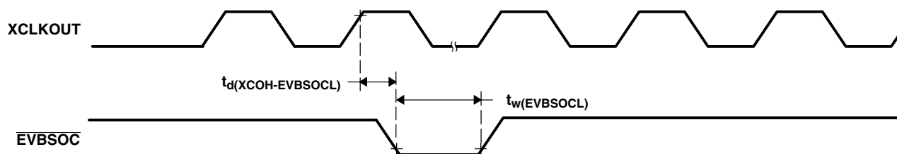
Figure 6–18. EVBSOC Timing
