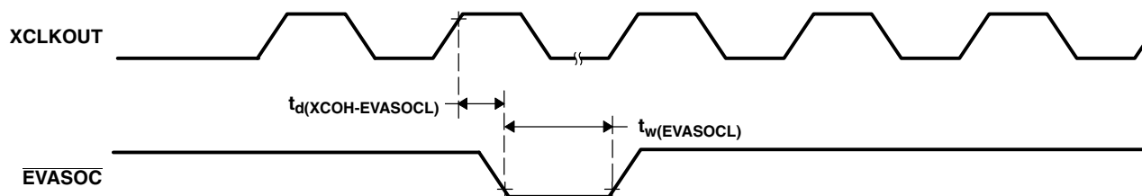
Figure 6–17. EVASOC Timing
