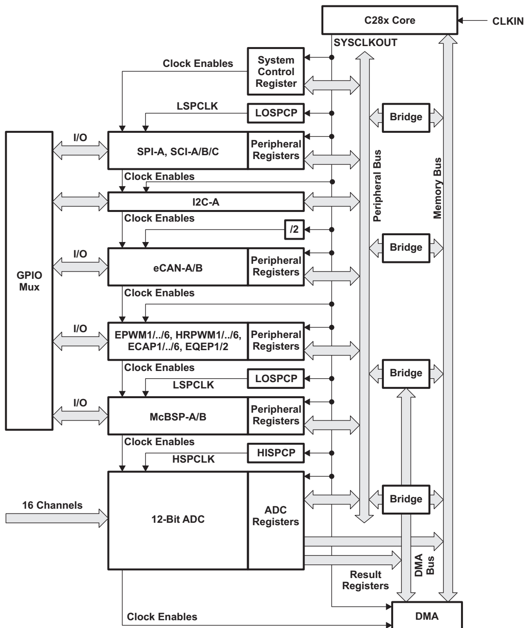
Figure 3-6. Clock and Reset Domains
