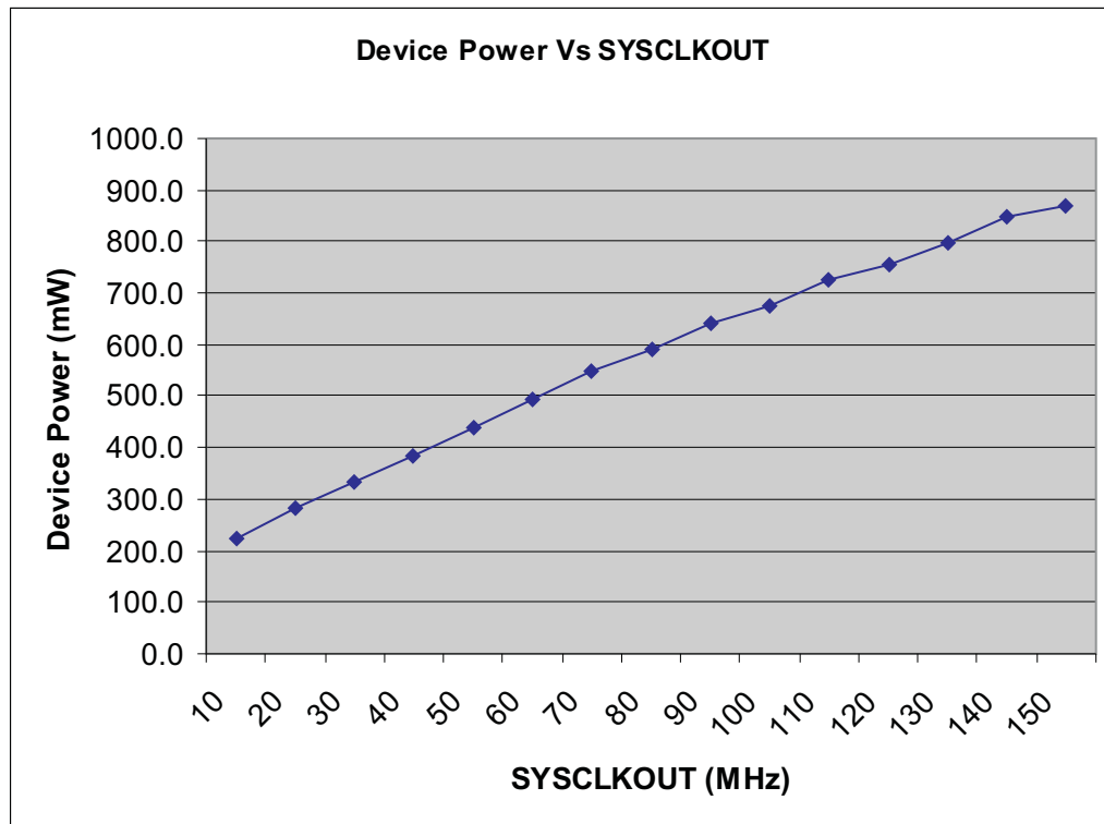
Figure 6-3. Typical Operational Power Versus Frequency
