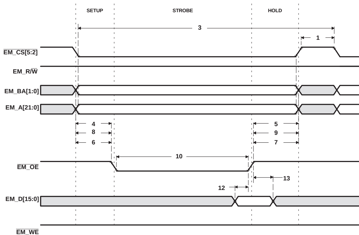
Figure 6-21. Asynchronous Memory Read Timing for EMIF
