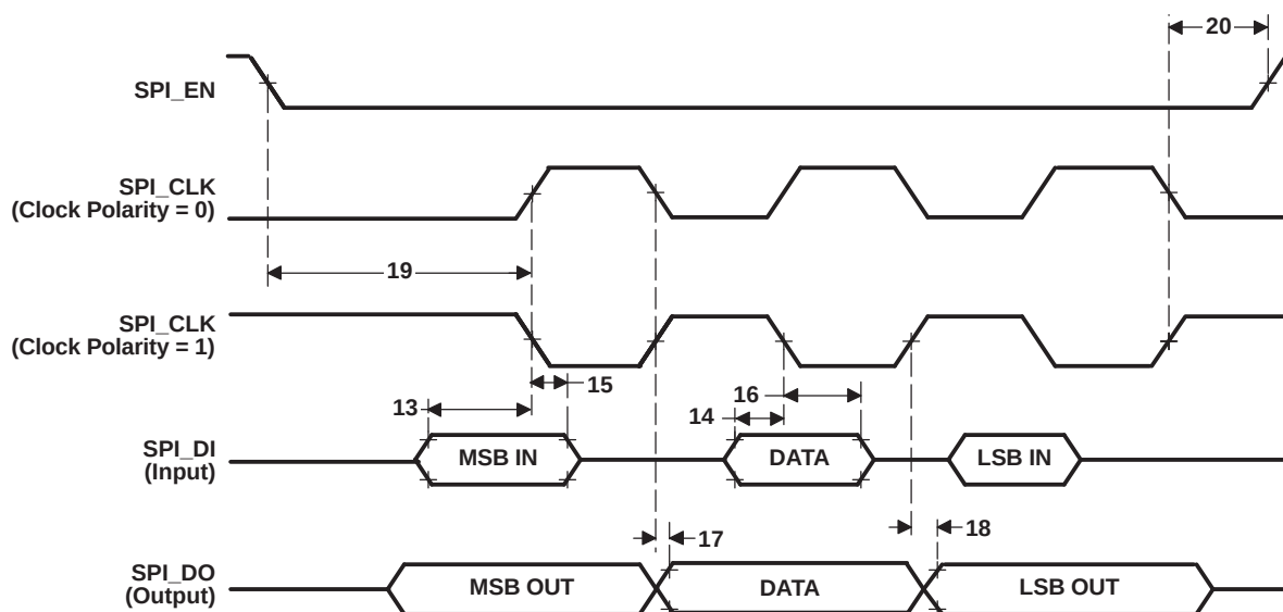
Figure 6-64. SPI Master Mode External Timing (Clock Phase = 1)
