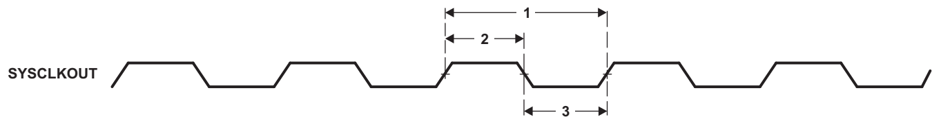
Figure 7-24. SYSCLKOUT Timing
