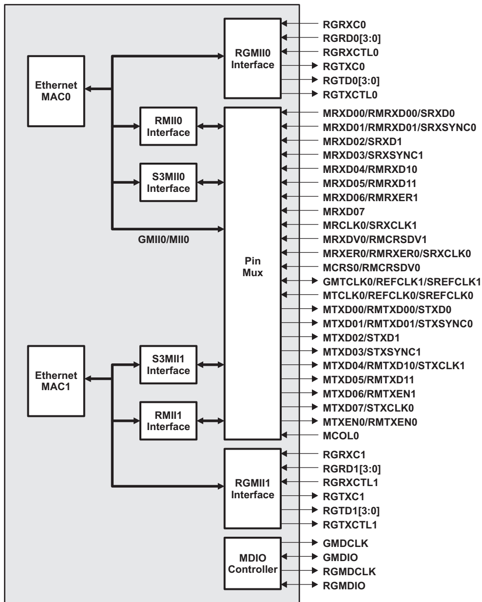
Figure 2-9. EMAC[1:0]/MDIO (RGMII[1:0], SGMII[1:0], MII0, RMII[1:0], and GMII0) Peripheral Signals
