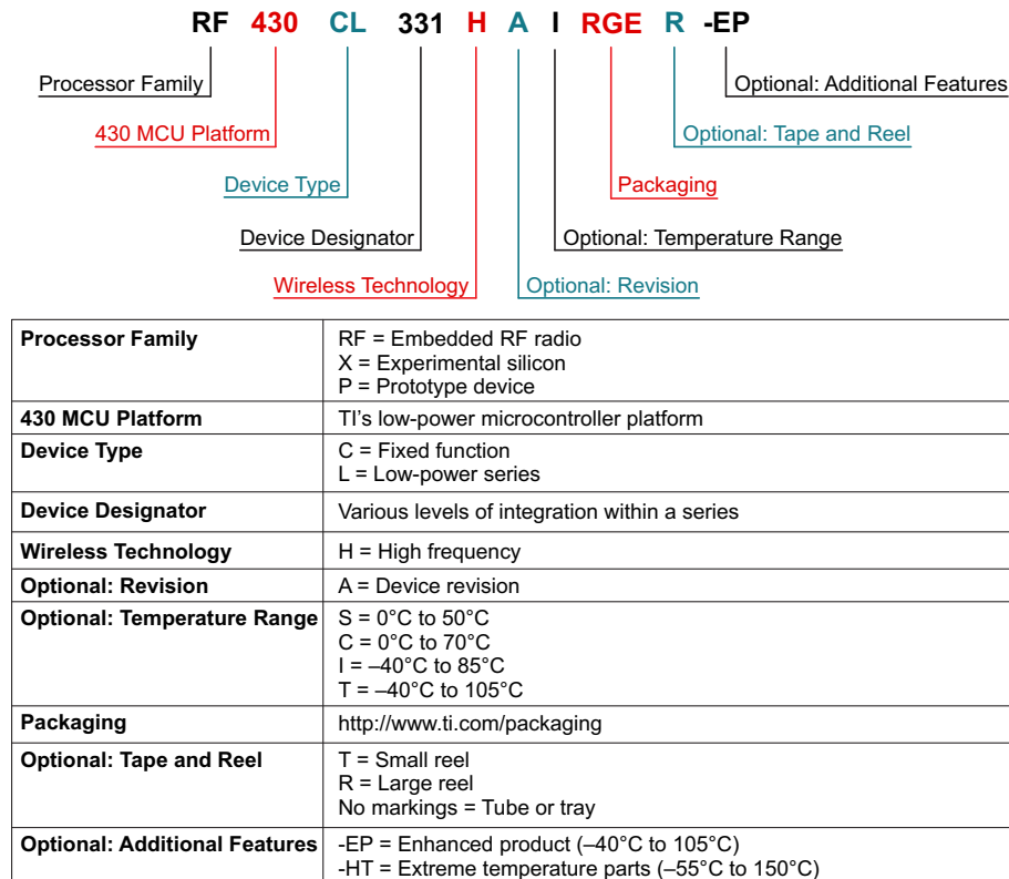
Figure 7-1. Device Nomenclature
