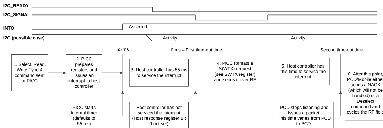
Figure 5-17. Timing Limits
