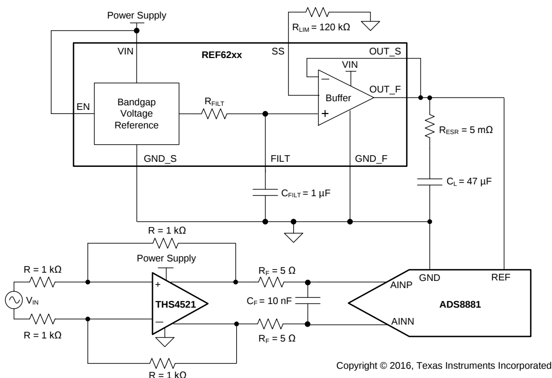
Figure 45. Burst-Mode Measurement Setup
