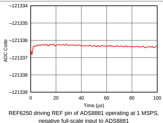
Figure 59. Reference Droop
