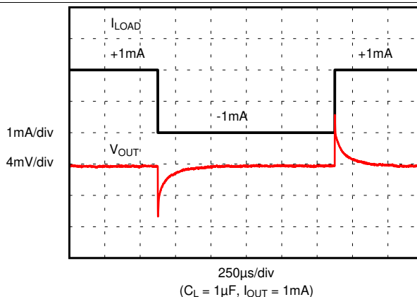
Figure 8. Load Transient
