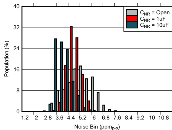
Figure 7-6. 0.1 Hz to 10 Hz Noise Distribution ( V_{REF} = 2.5\text{ V} , C_L = 1\text{ }\mu\text{F} , I_L = 0\text{ mA} )
