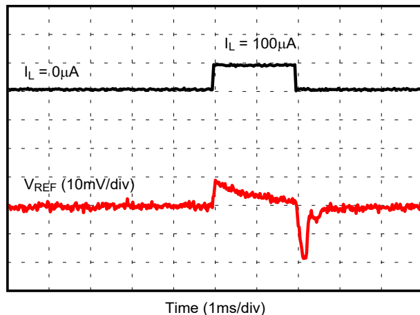
Figure 9-3. Load Transient Response 0 \mu\text{A} to 100 \mu\text{A} , C_{REF} = 1 \mu\text{F}
