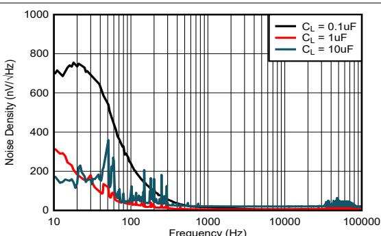
Figure 8-12. Noise Spectrum 10 Hz to 100 kHz ( V_{REF} = 2.5\text{ V} )
