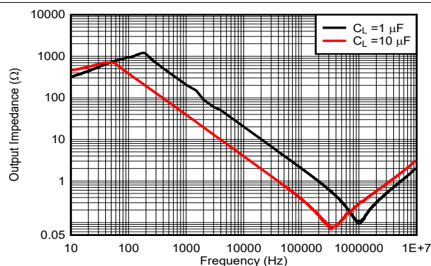
Figure 7-23. Output Impedance
