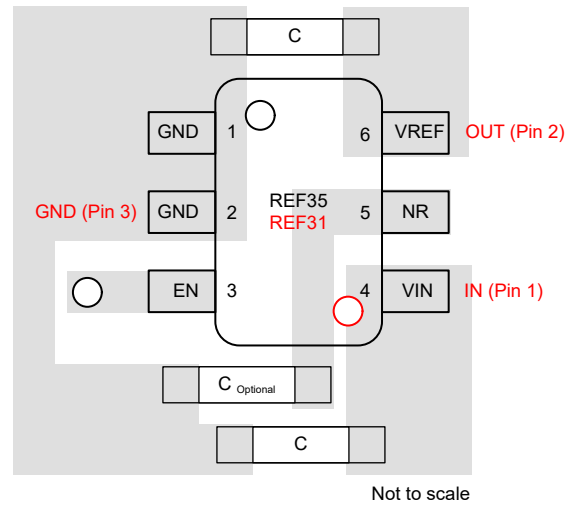
Figure 10-4. Pin Compatibility With REF31xx
