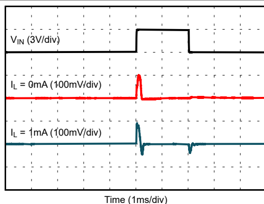
Figure 7-21. Line Transient Response ( V_{REF} = 2.5\text{ V} , C_L = 1\text{ }\mu\text{F} )
