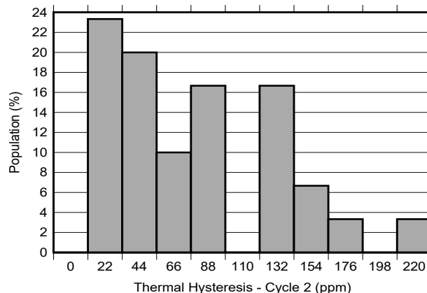
Figure 8-6. Thermal Hysteresis Distribution -40°C to 125°C, Cycle 2
