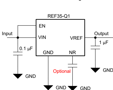
Connection Diagram
