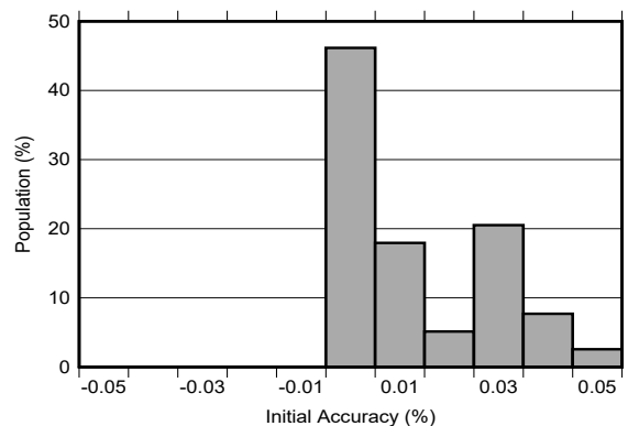
Figure 7-2. Initial Accuracy Distribution
