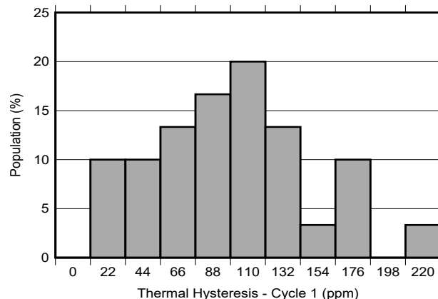
Figure 8-5. Thermal Hysteresis Distribution -40°C to 125°C, Cycle 1
