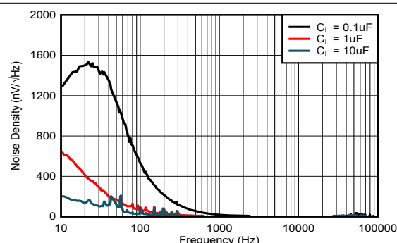
Figure 8-13. Noise Spectrum 10 Hz to 100 kHz ( V_{REF} = 5\text{ V} )
