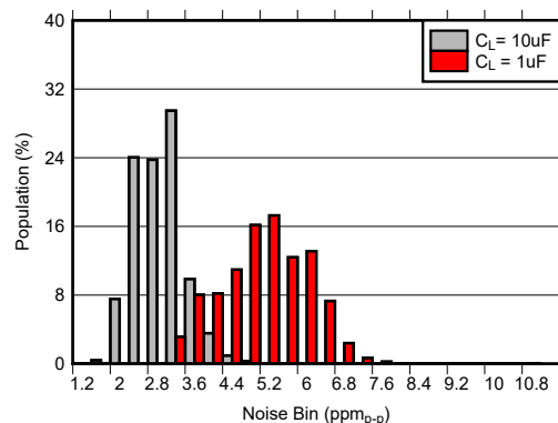
Figure 7-4. 0.1 Hz to 10 Hz Noise Distribution ( V_{REF} = 2.5\text{ V} , C_{NR} = \text{Open} , I_L = 0\text{ mA} )
