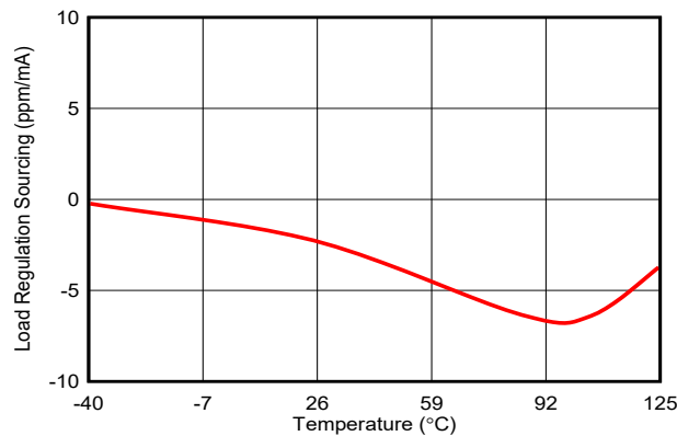
Figure 7-11. Load Regulation (Sourcing 10 mA) vs Free-Air Temperature
