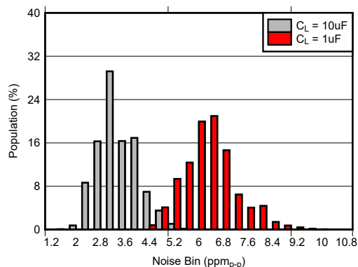
Figure 7-3. 0.1 Hz to 10 Hz Noise Distribution ( V_{REF} = 1.25\text{ V} , C_{NR} = \text{Open} , I_L = 0\text{ mA} )
