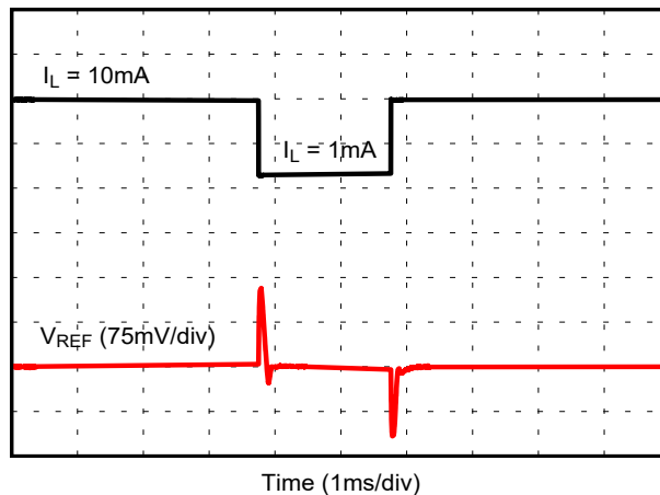
Figure 9-4. Load Transient Response 1 mA to 10 mA, C_{REF} = 1 \mu\text{F}
