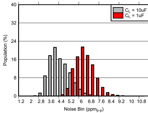
Figure 7-7. 0.1 Hz to 10 Hz Noise Distribution ( V_{REF} = 5\text{ V} , C_{NR} = \text{Open} , I_L = 0\text{ mA} )
