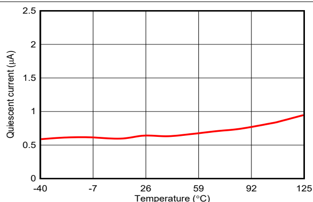
Figure 7-24. Quiescent Current vs Free-Air Temperature
