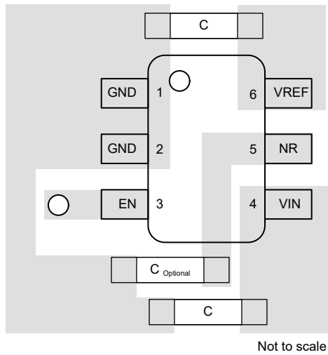
Figure 10-3. Layout Example
