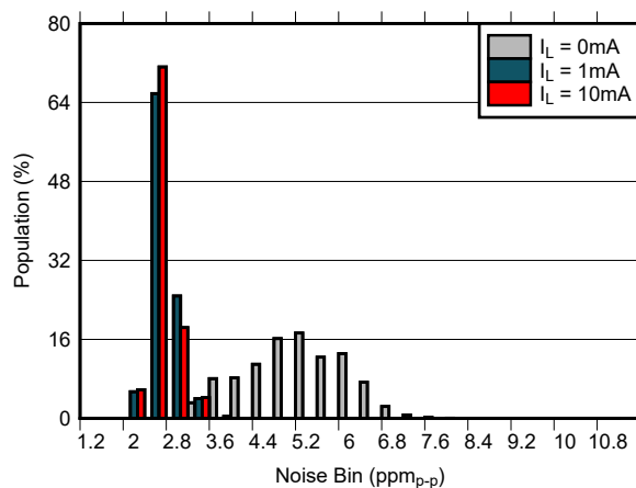
Figure 7-5. 0.1 Hz to 10 Hz Noise Distribution ( V_{REF} = 2.5\text{ V} , C_L = 1\text{ }\mu\text{F} , C_{NR} = \text{Open} )
