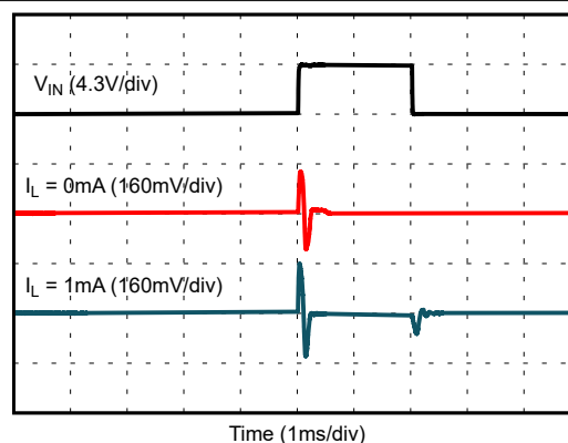
Figure 7-20. Line Transient Response ( V_{REF} = 1.25\text{ V} , C_L = 1\text{ }\mu\text{F} )
