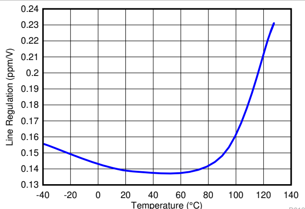
Figure 7-6. Line Regulation
