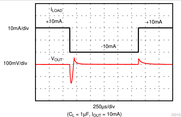
Figure 6-12. Load Transient
