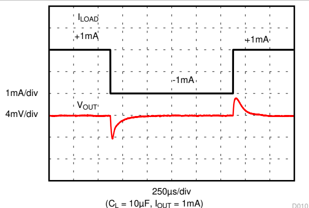
Figure 6-11. Load Transient
