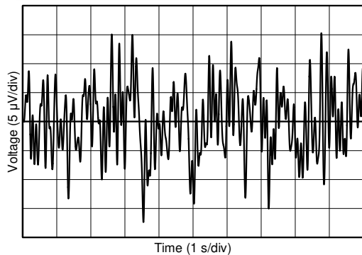
Figure 8-7. 0.1-Hz to 10-Hz Noise ( V_{\text{REF}} )
