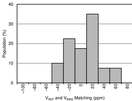
Figure 10-4. V_{REF} - 2 \times V_{BIAS} Distribution (At T_A = 25^\circ\text{C} )
