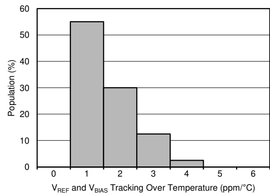
Figure 10-5. Distribution of V_{REF} - 2 \times V_{BIAS} Drift Tracking Over Temperature
