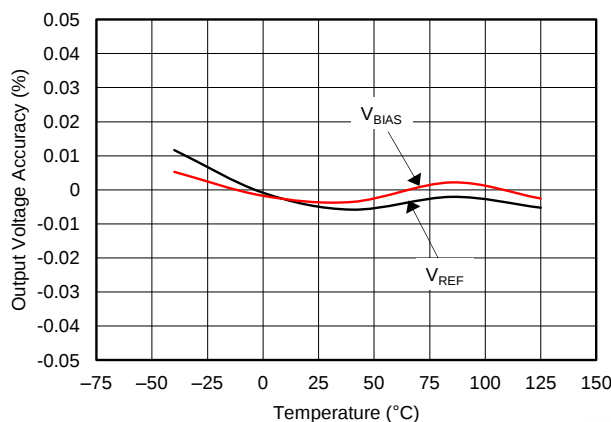
Figure 44. V REF and V BIAS Tracking vs Temperature
