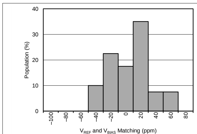
Figure 48. V_{REF} - 2 \times V_{BIAS} Distribution (At T_A = 25^\circ\text{C} )
