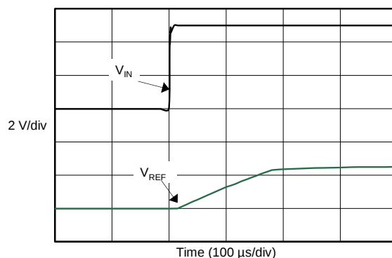
Figure 26. Turn-On Settling Time
