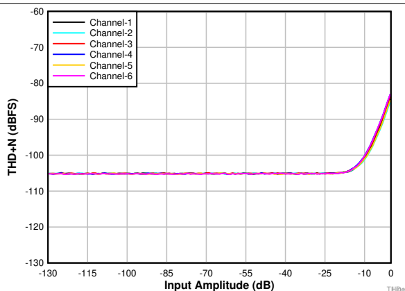
Figure 5. THD+N vs Input Amplitude
