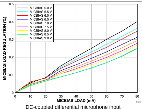
Figure 18. MICBIAS Load Regulation vs MICBIAS Load Current
