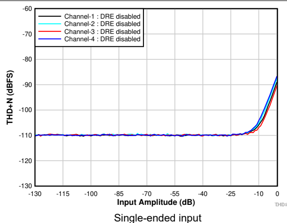
Figure 6-8. THD+N vs Input Amplitude With DRE Disabled
