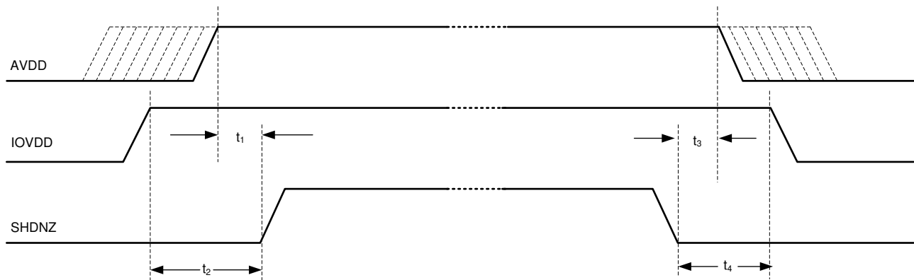
Figure 9-7. Power-Supply Sequencing Requirement Timing Diagram
